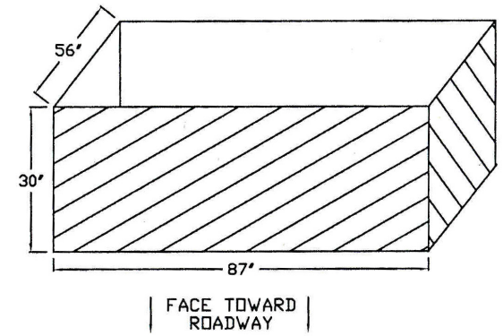
MINIMUM EXCAVATION REQUIREMENTS
